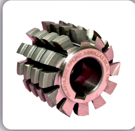
Spline Hob Cutter
